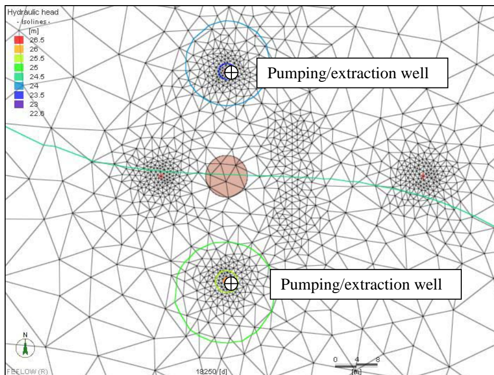
Figure 32. Hydraulic heads at the end of the simulation period (50 years) – bidirectional scenario
