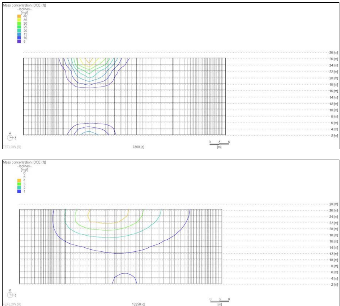
Figure 26. West-East cross-sectional view of DCE groundwater concentration isolines at the start of the GWE-system (top) and at the end of the simulation period (50 years) (below) – GWE with groundwater containment
